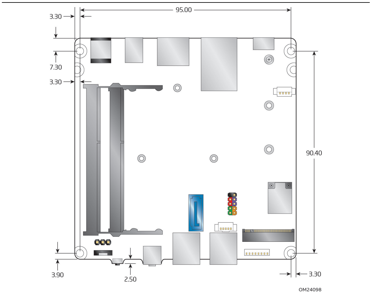
Figure 16. Board Dimensions
